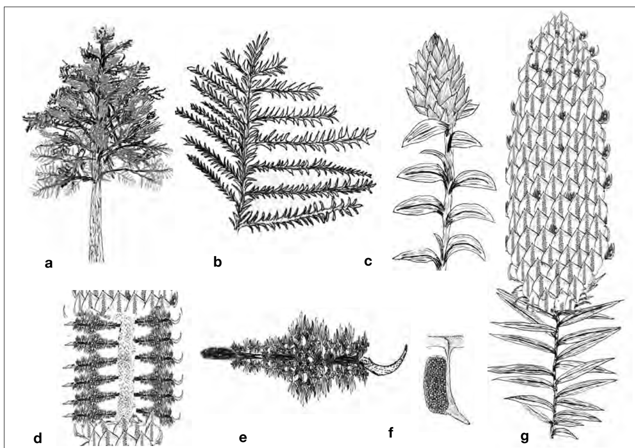
Albertia alpina – Suggested reconstruction of the conifer: a) whole plant, b) juvenile sterile shoot, c) Pusterostrobus haidingeri , immature female cone of Albertia alpina , d) Darneya schaurothi , part of a male cone with attached microsporophylls (PIZ 603), e) Darneya schaurothi - male fructification showing the attachment of pollen clusters, f) Darneya schaurothi , single pollen sac, g) Darneya schaurothi , entire male cone (PIZ 583)
