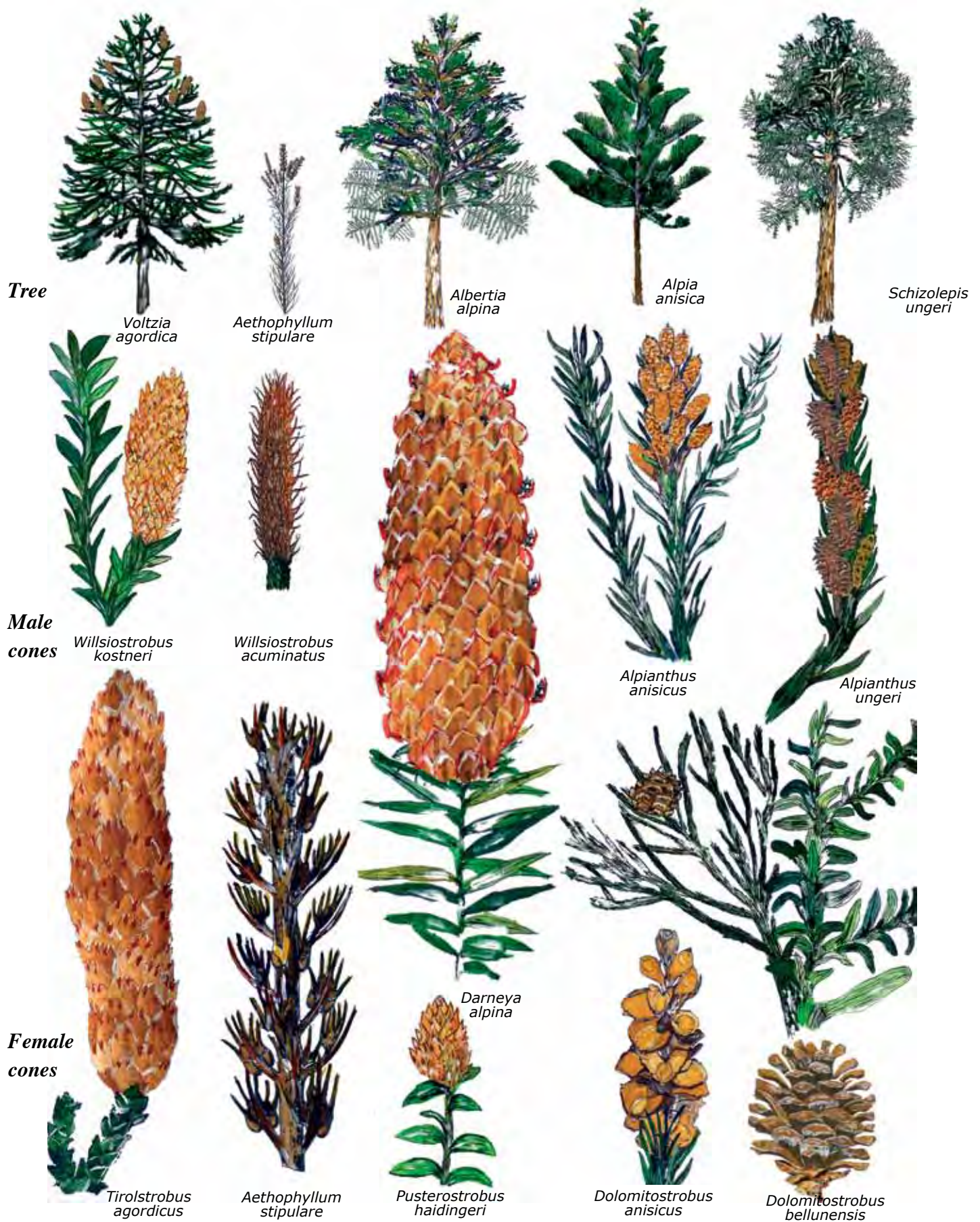
Reconstruction of the Early-Middle Mesozoic coniferales from the Dolomites: Voltzia agordica , Aethophyllum stipulare (after Grauvogel-Stamm), Albertia alpina , Alpia anisica , Schizolepis ungeri . Male and female cones, half their natural size.
