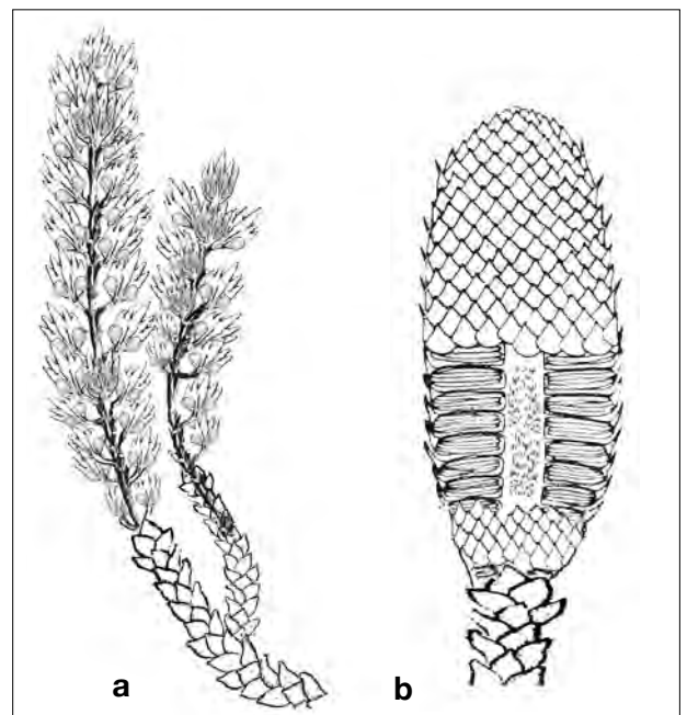
Voltzia unescoensis . a) Suggested reconstruction of a young female cone (KÜH 365) b) Willsiostrobus unescoensis . Male cone of Voltzia unescoensis (KÜH 1193)
