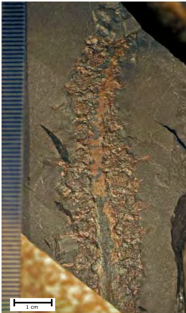
Suggested male cone of Albertia/Darneya from the lower Rotliegend (Lower Permian), Steinbruch Cabarz, near Tabarz, Germany (Collection Stephan Brauner WP 5924, classified as a conifer shoot). Courtesy of the Natural History Museum Schloss Bertholdsburg Schleusingen.
