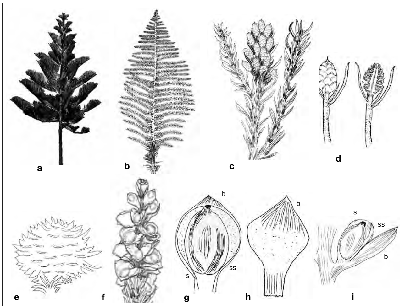
Alpia anisica – Suggested reconstruction of the conifer: a) whole tree, b) complete twig, c) Alpianthus anisicus – male cone of Alpia anisica (PIZ 42), d) male cone with detail of the pollen sacs, e) Dolomitostrobus anisicus – immature female cone (KÜH 1249), f) Dolomitostrobus anisicus – decaying adult female cone (PIZ 514), g) Seed-scale interior, h) Bract-scale: outer side, i) Bract-scale: lateral side (ss = seed-scale, s = seed, b = bract-scale)
