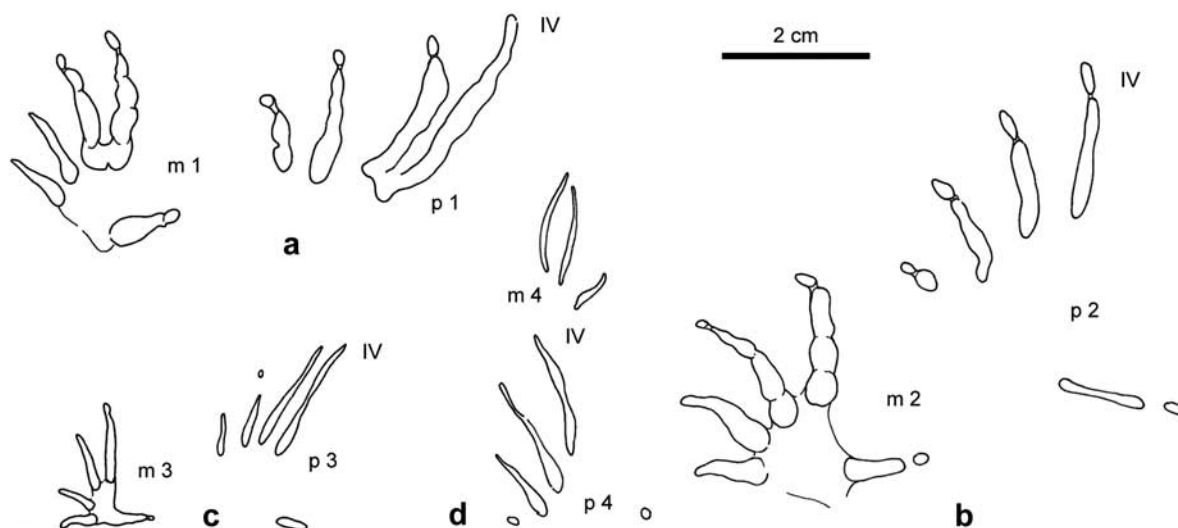
Fig. 2: Rhynchosauroides footprints types from Piz da Peres ichnosite (m: manus, p: pes).
